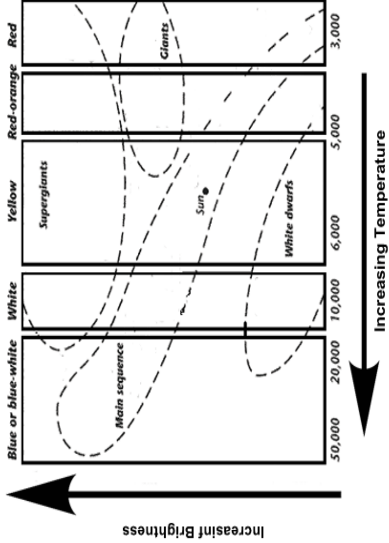
Hertzsprung-Russell Diagram
